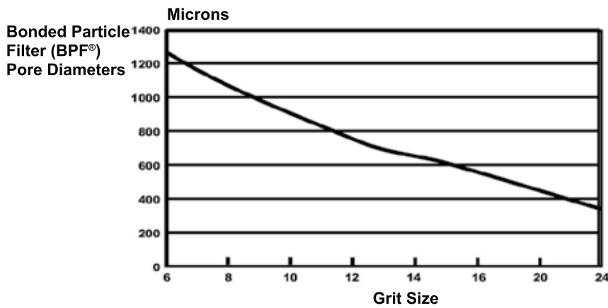
Figure 1 - Pore Diameters
